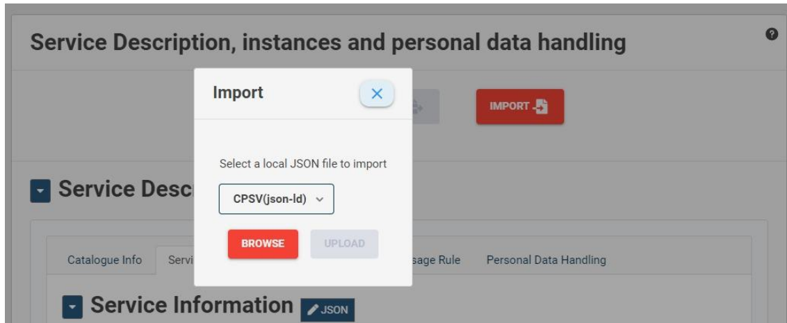
Figure 24 - Import dialog
