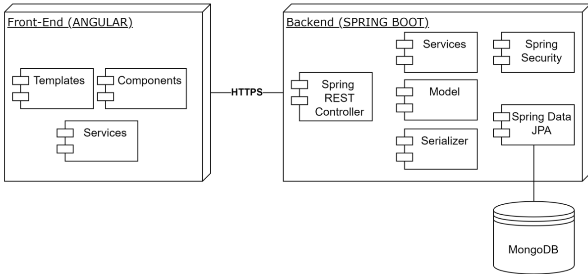
Figure 14 - Front-End and Backend of Service Catalogue implementation
