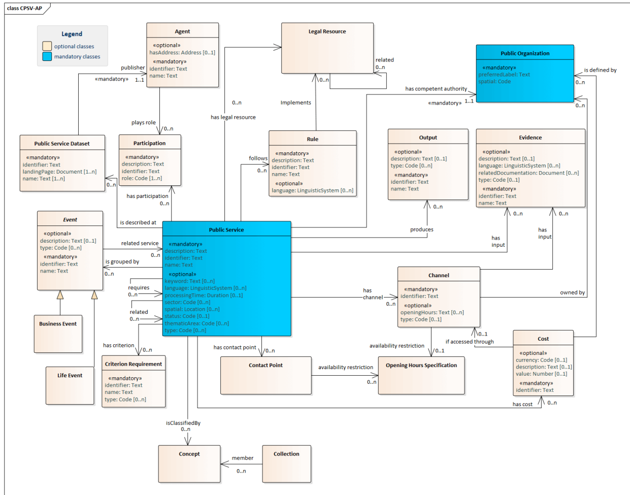
Figure 10 - Graphical representation of the relationships between the classes and properties of the full Core Public Service Vocabulary Application Profile ( figure from [2])
