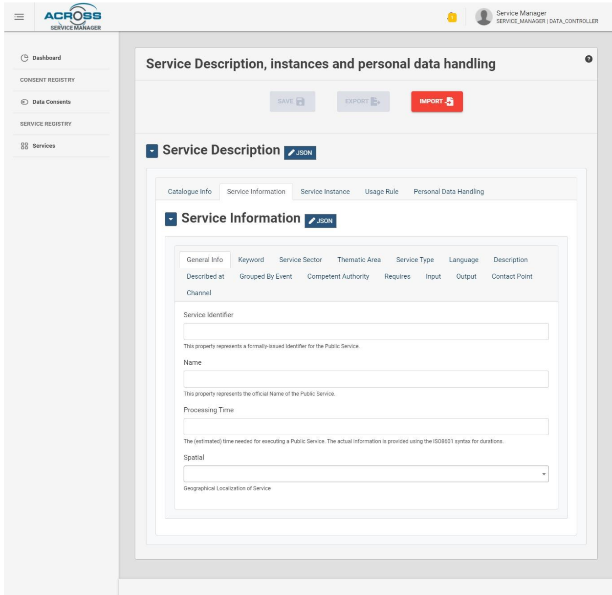
Figure 23 - Service Editor page
