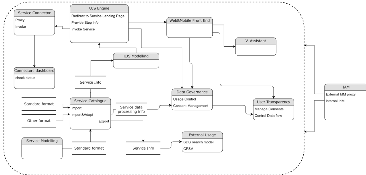
Figure 8 - Service Catalogue and Service Adapted modules interaction map with other modules of ACROSS platform.
