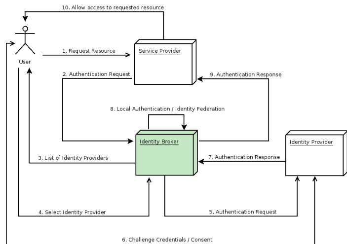
Figure 17 - Identity brokering flow supported by Keycloak
