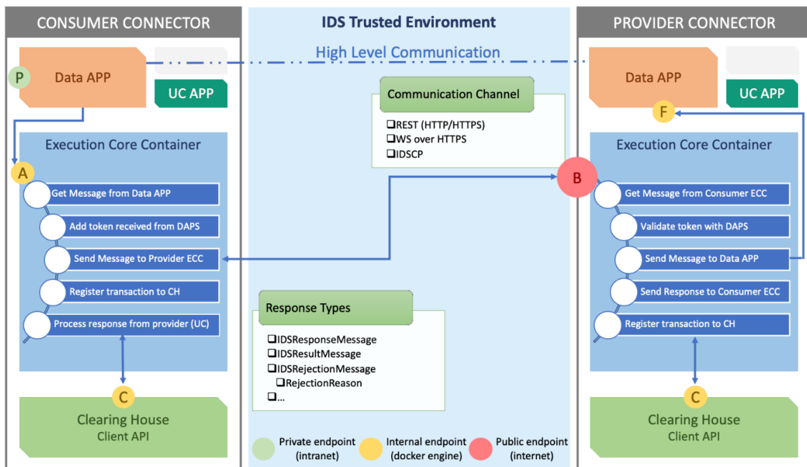
Figure 29 - TRUE Connector Architecture and Interactions
