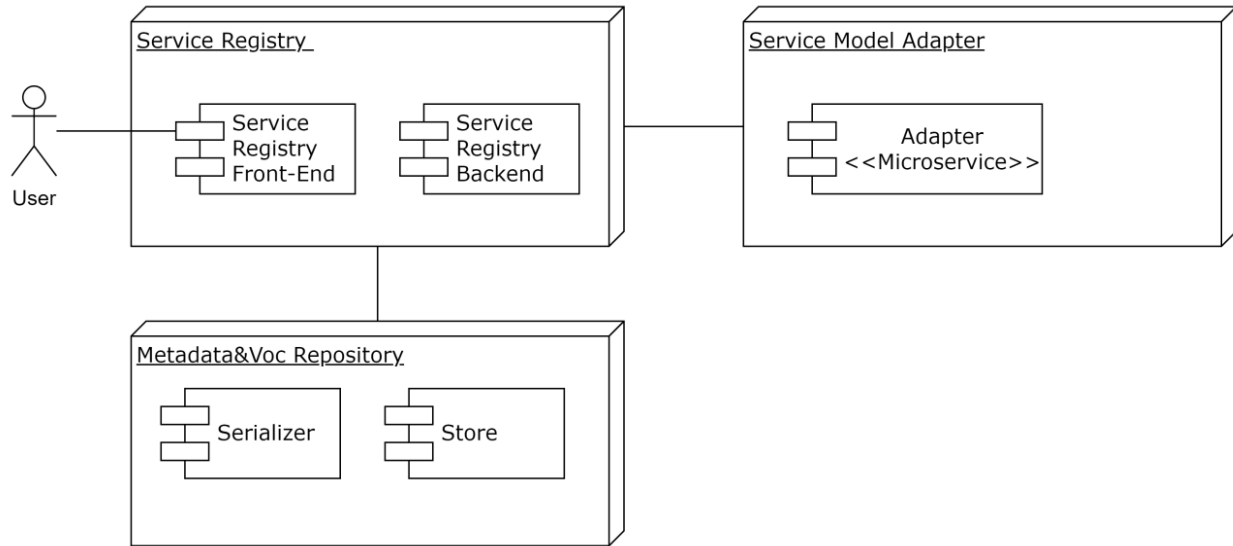
Figure 13 - Main modules implemented by the Service Catalogue
