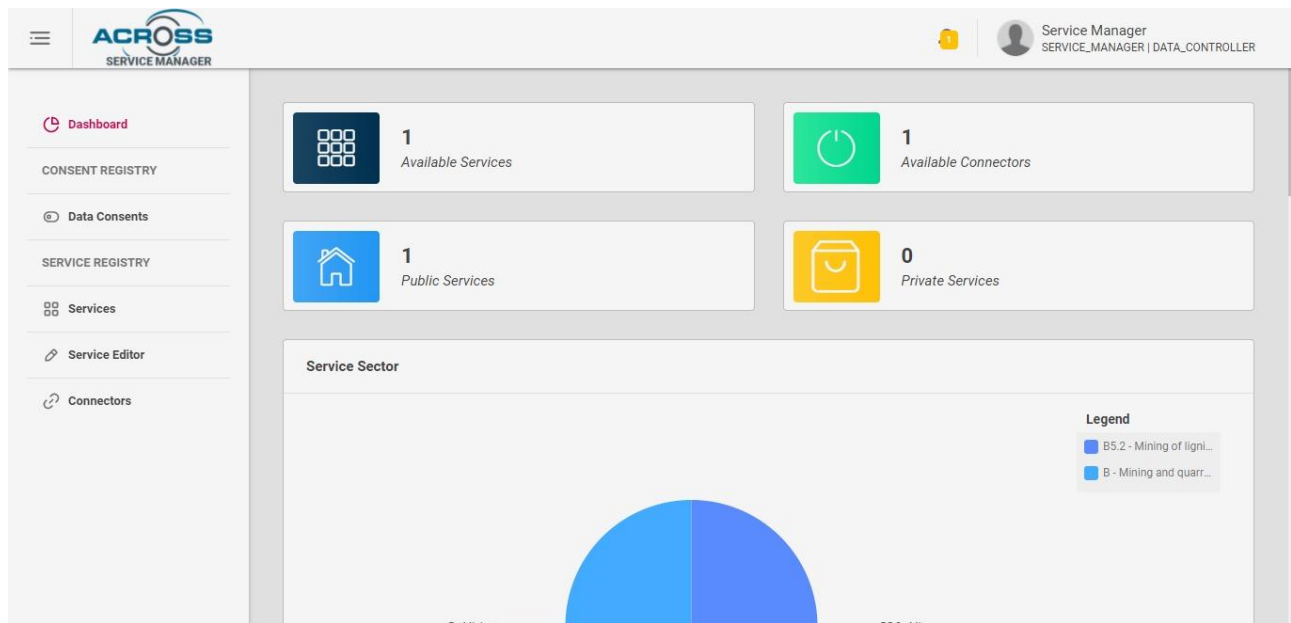
Figure 27 - Dashboard page
