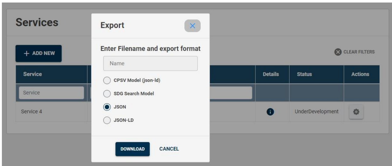
Figure 22 - Export dialog
